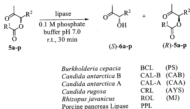
Scheme 2. Enzymatic resolution of acyloin esters 5 with commercial lipases and their abbreviations (in brackets: alternative abbreviations commonly used)
