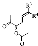
Figure 1. Acyloin substrate model for BCL
