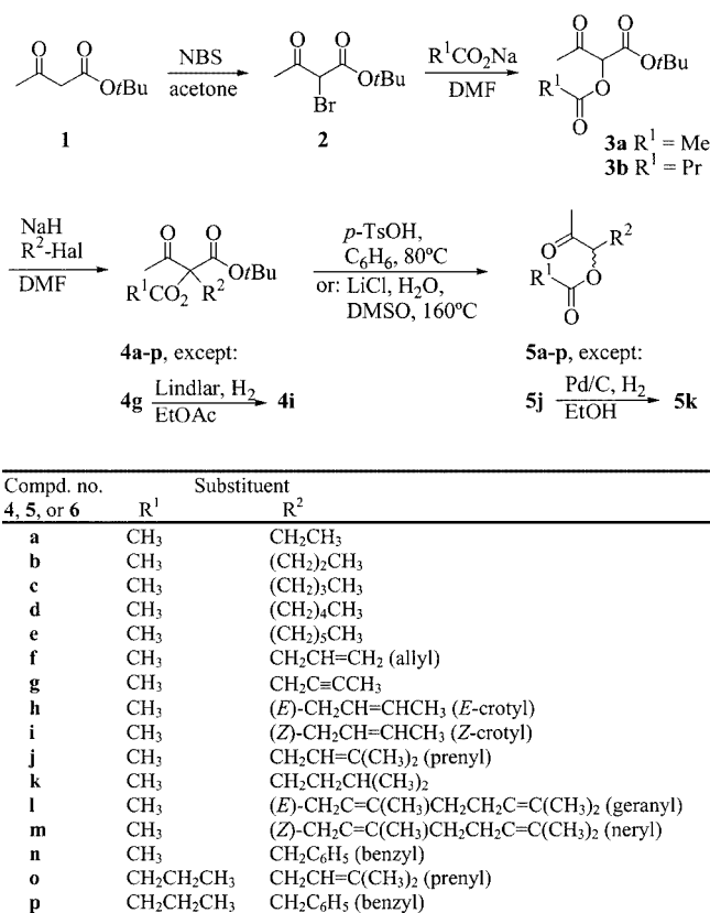
Scheme 1. Synthesis of acyloin esters 5 and acyloins 6 from acetoacetate
